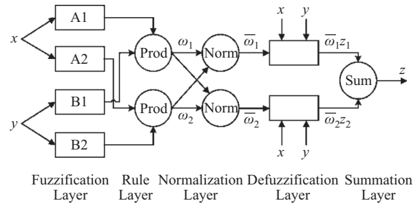
Fig. 1. ANFIS architecture [35].
